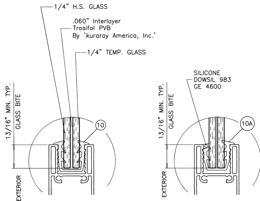
ALT. GLAZING GASKET
